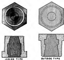
Figs. 234-236. Fusible Plugs.
